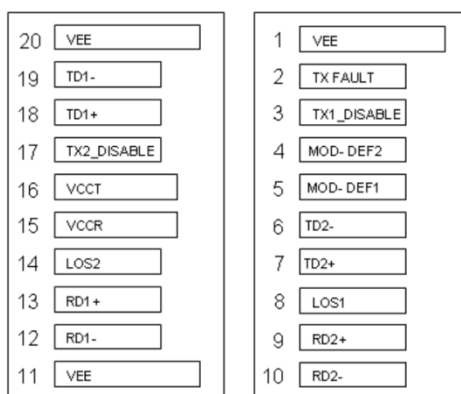
Top view of Board
